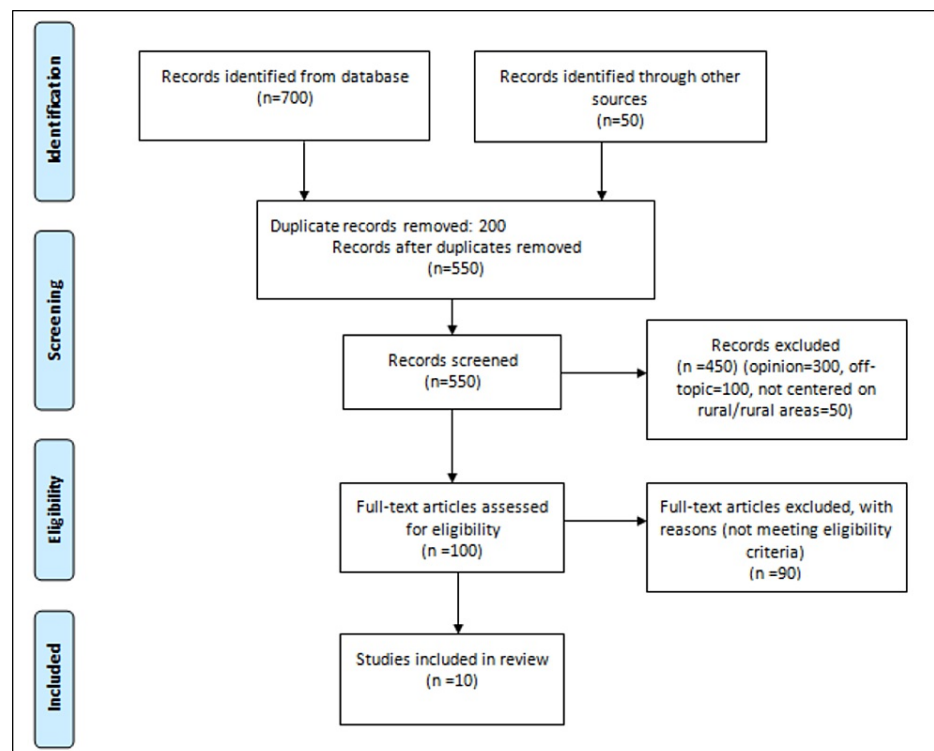
FIGURE 1: PRISMA diagram
